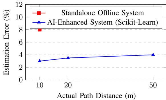
Fig. 1. Distance estimation error comparison between Standalone and AI-Enhanced systems.
