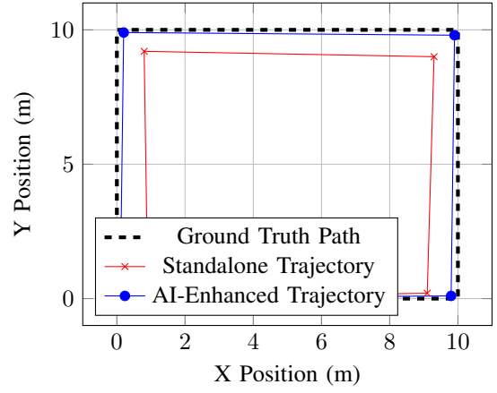
Fig. 2. 2D Indoor tracking and trajectory mapping reconstruction for a 10 m \times 10 m closed-loop test course.
